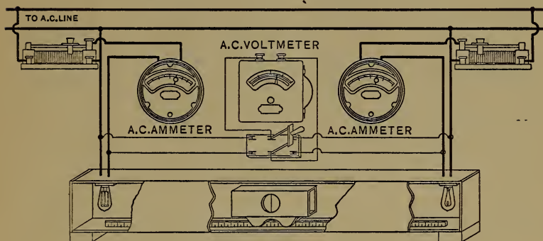
FIG. 10.—AN EXERCISE IN PHOTOMETRY. Fee's Method.
